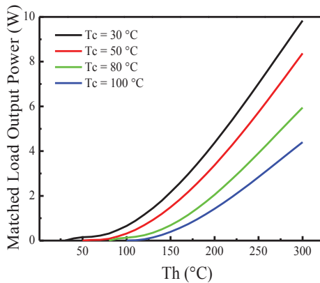
The chart for matched load output power Vs Th under various Tc
